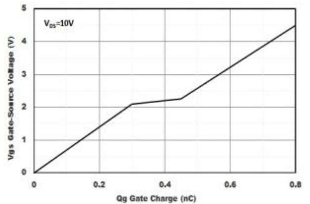
Gate Charge
